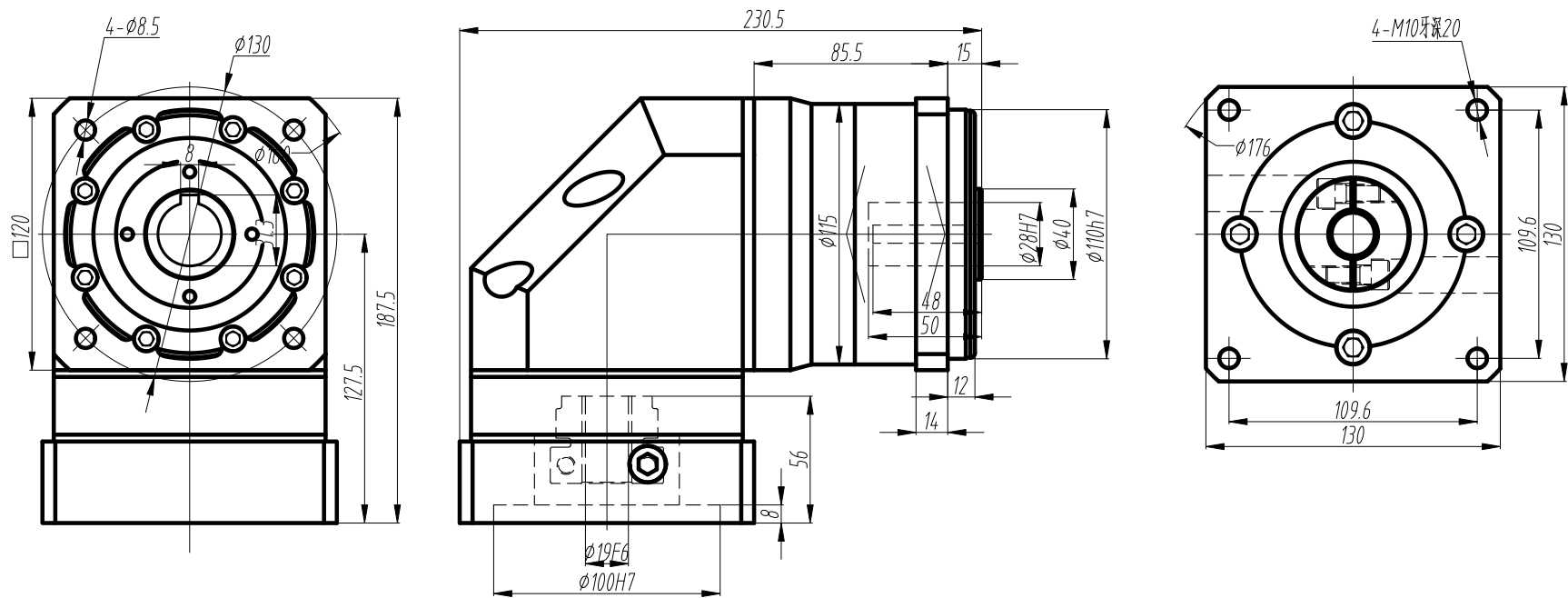
标准轴 Standard output shaft
